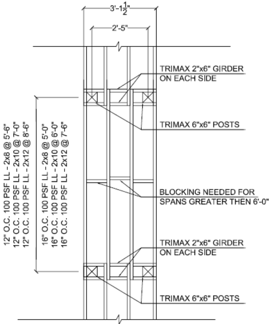
Commercial Boardwalk Design Designed for TRIMAX Structural Lumber 3'-0" Wide Boardwalk Layout 100 PSF Live Load \frac{1}{2}'' = 1'-0''
