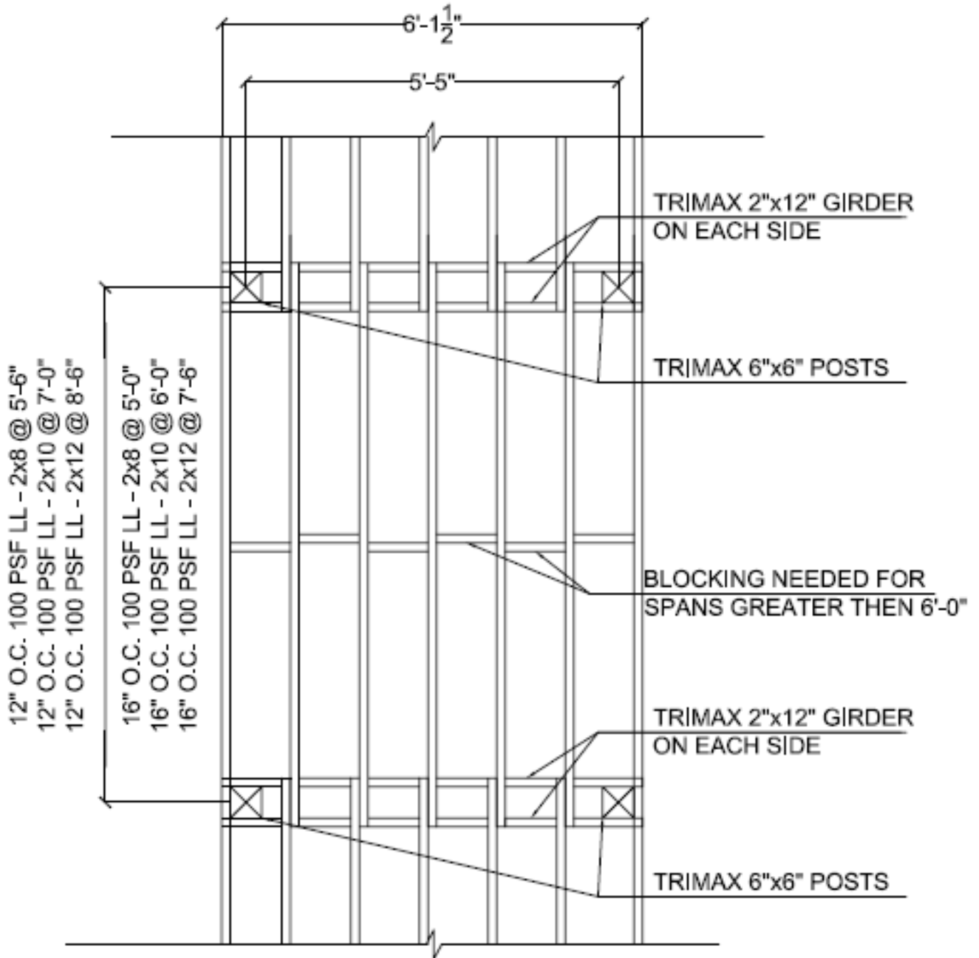
Commercial Boardwalk Design Designed for TRIMAX Structural Lumber 6'-0" Wide Boardwalk Layout 100 PSF Live Load \frac{1}{2} " = 1'-0"
