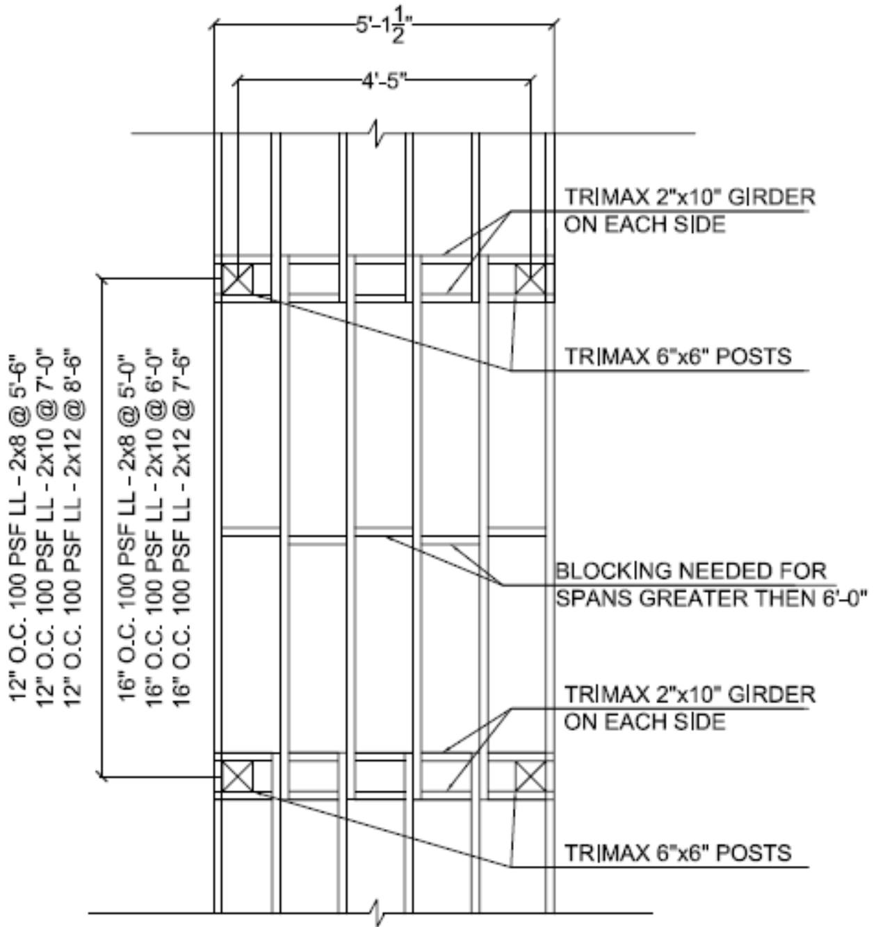
Commercial Boardwalk Design Designed for TRIMAX Structural Lumber 5'-0" Wide Boardwalk Layout 100 PSF Live Load 1/2" = 1'-0"
